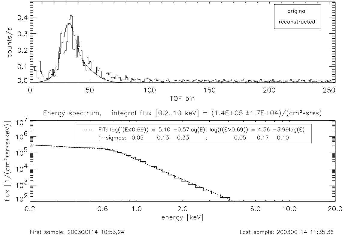
Fig. 3.— Example of a TOF spectrum for 2003 October 14, from NPD1, channel 0. Every incoming ENA is stored as a single count in one of the 256 TOF bins, each 8 nanoseconds wide. The top panel shows the original TOF spectrum (accumulated for 2000 s) and the reconstructed TOF signal after background removal and noise filtering. The bottom panel shows the energy spectrum calculated from the reconstructed TOF signal above, and a fit to this spectrum (dotted line).
